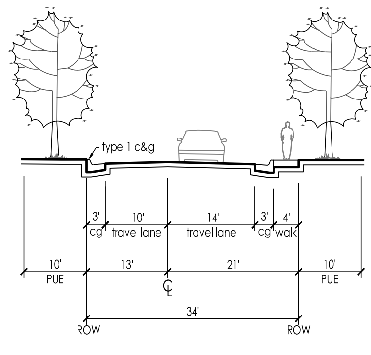
E MINOR RESIDENTIAL STREET (NO PARKING WEST SIDE) n.t.s.
